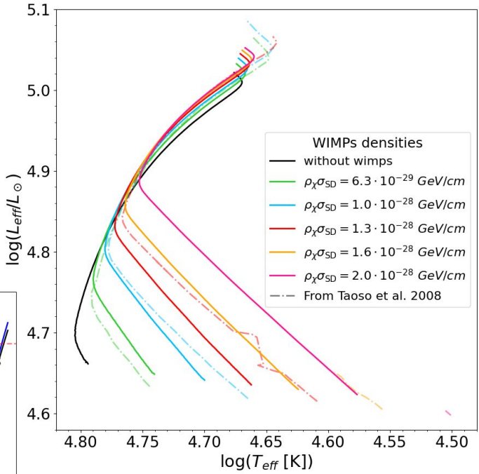
Hertzsprung-Russell diagram of a 20 M ⊙ with different WIMP densities →
