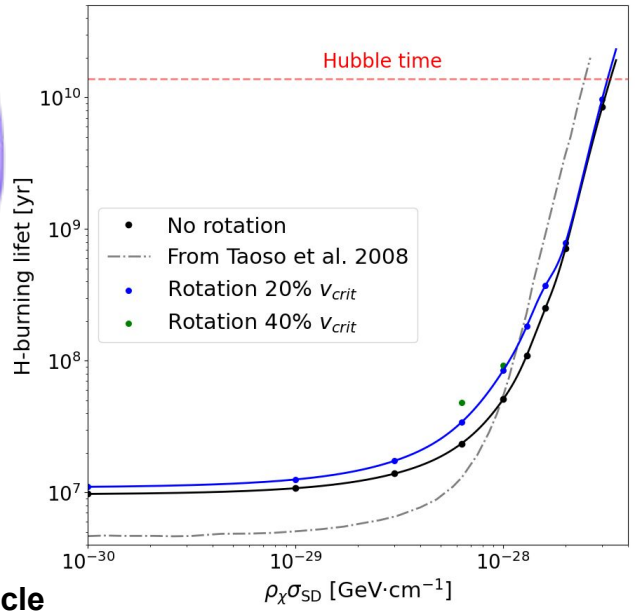
← Main Sequence lifetime as a function of WIMP densities, for different rotation velocities
